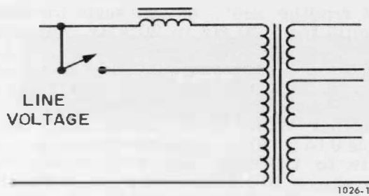
Figure 12. Elementary schematic showing pre-regulator tap-switching scheme.
