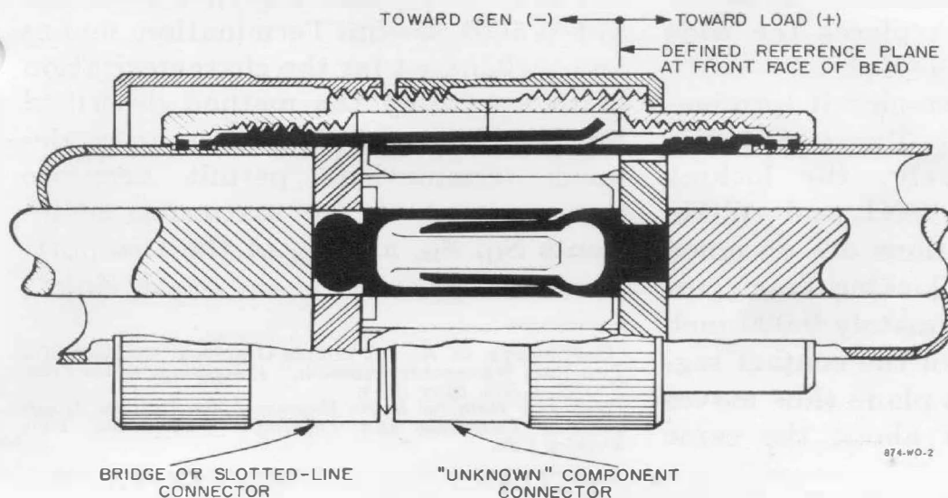
Figure 2. Cross-section of mated GR874 connectors defining reference plane.
