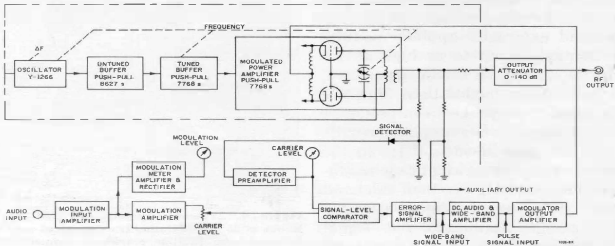
Figure 5. Elementary block diagram.
