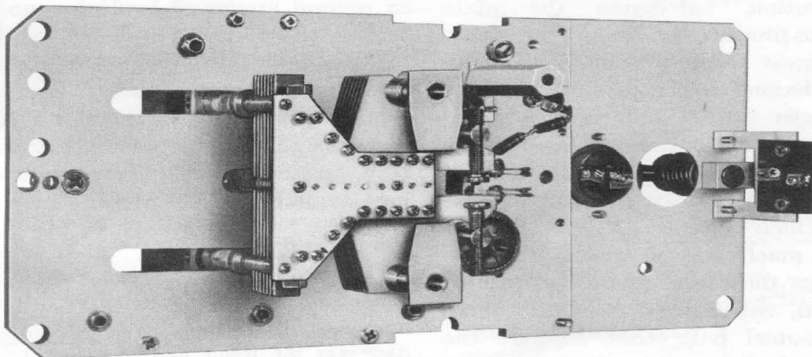
Figure 1. The guillotine capacitor, as used in the 1026 Standard-Signal Generator.
