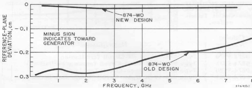
Figure 3. Typical reference-plane-deviation vs frequency for old and new Type 874-WO Open-Circuit Terminations.
