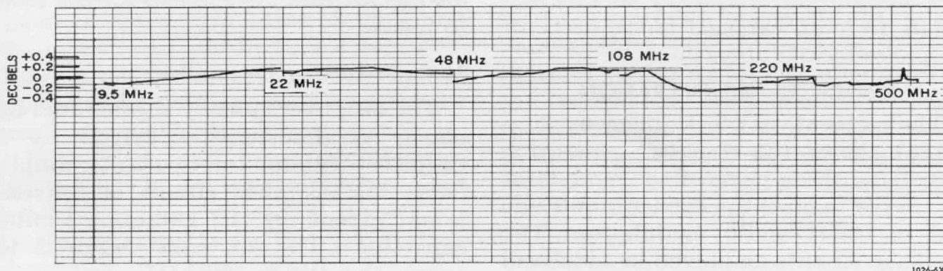
Figure 3. Output level vs carrier frequency. The small discontinuities in level (typically less than 0.2 dB) occur at frequencies where the range is changed.
