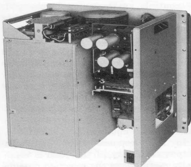
Figure 2. Rear interior view.
