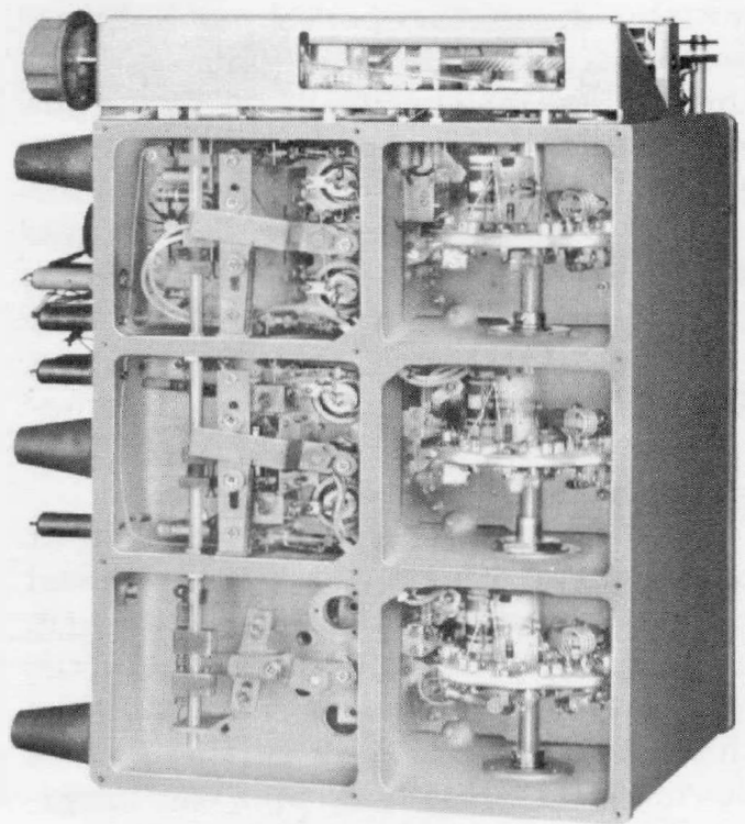
Figure 6. Side interior view. The ganged turrets for the three tuned stages are in the right-hand compartments; the tube sockets for the amplifier and tuned buffer stages are visible in the upper two left-hand compartments.
