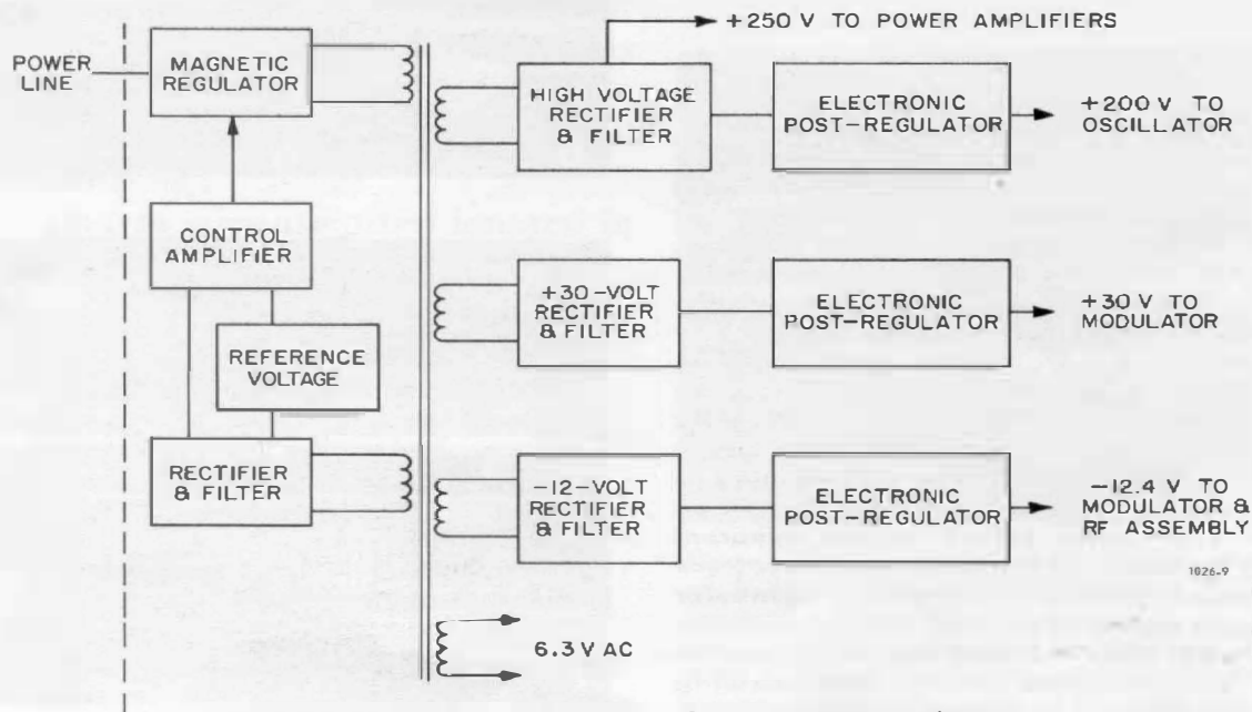
Figure 11. Block diagram of the power supply.
