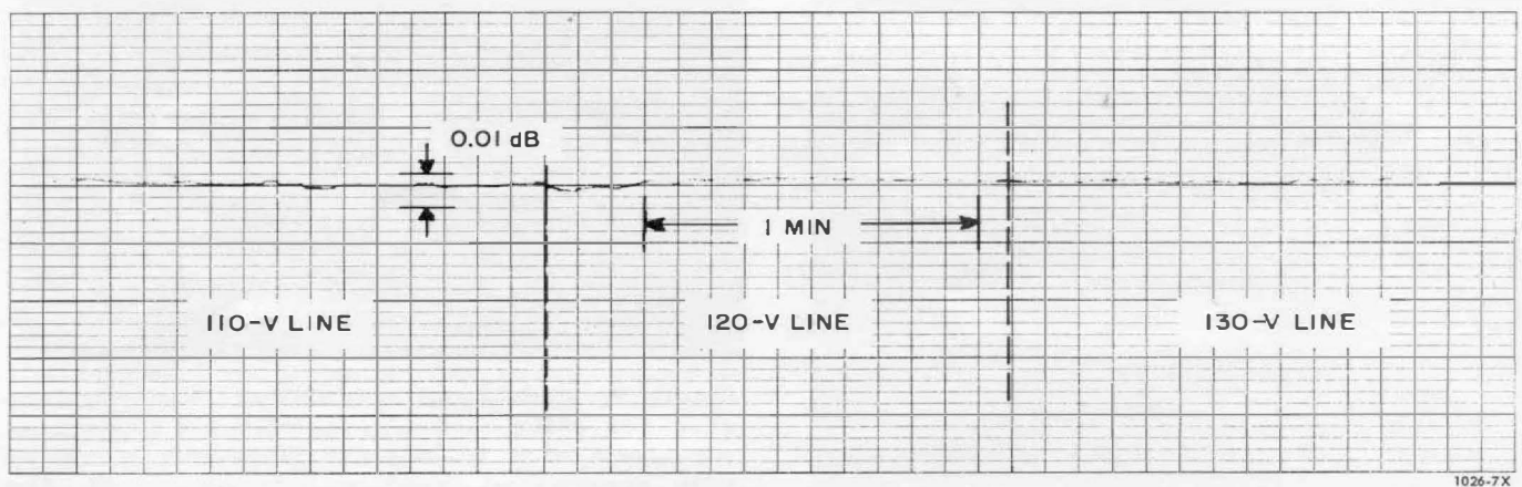
Figure 7. Short-term amplitude stability. The peak amplitude of the envelope of a 400-MHz carrier modulated 95% at 1 kHz, recorded against time with line-voltage steps.
