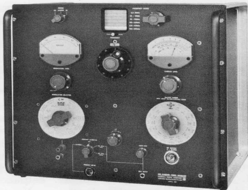
Figure 1. The 1026 Standard-Signal Generator.
