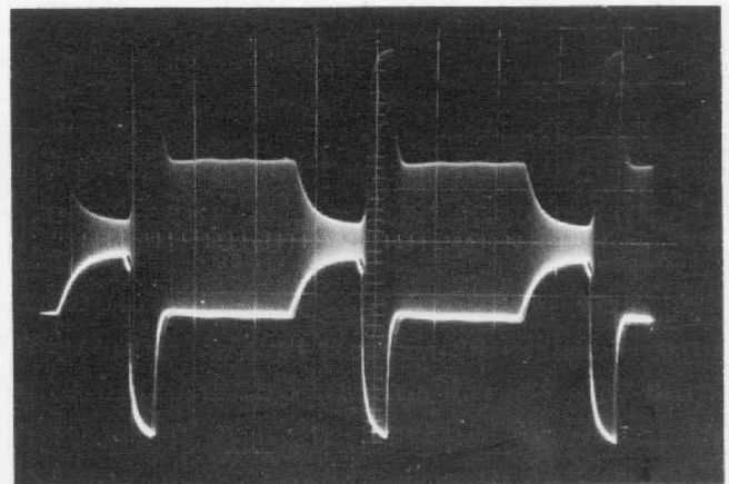
Figure 9. Wide-band modulation: The envelope of a 400-MHz carrier modulated by a complex waveform at a 50-kHz repetition rate is shown with superposed input modulation signal. The 2- \mu s-duration modulation peak is produced by the negative-going portion of the input signal.
