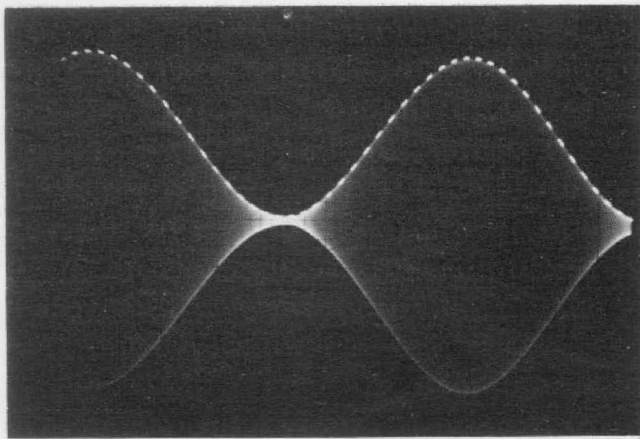
Figure 8. Modulation linearity: The envelope of a 400-MHz carrier modulated 95% at 1 kHz is shown with superposed modulation signal. The oscilloscope trace of the 1-kHz modulation signal has been intensity-modulated at a synchronized 30-kHz rate to avoid masking of the modulation envelope.
